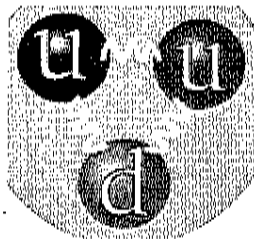
three quarks
